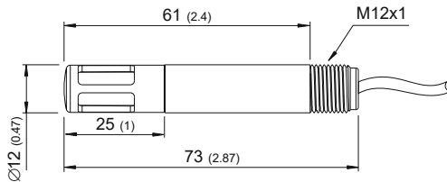
Fig. 1 Dimensions of EE08 in mm (inch)
